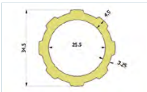
Non-slip rungs through profiling
